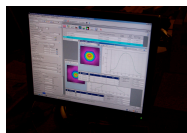
SOFTWARE
